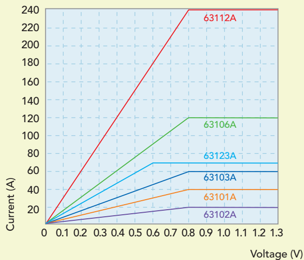
低电压特性 (Typical) 型号 63101A/63102A/63103A/63106A/63112A/63123A
