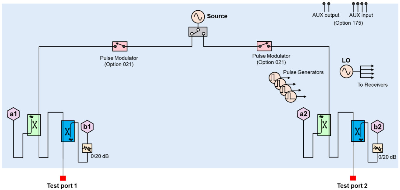
E5080B Option 2L0/2M0/2N0/2P0 (2-port base options)
