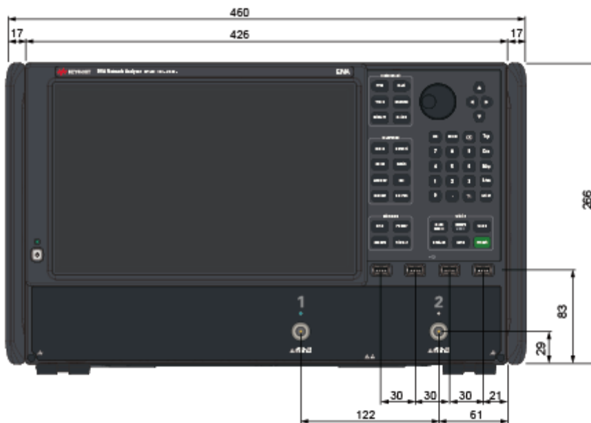
Dimensions (front view, E5080B with option 240/260/290 (Type-N), in millimeters)
