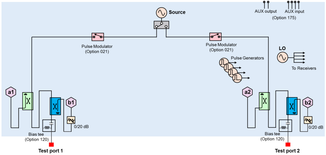
E5080B Option 240/260/290/2D0/2K0 (2-port base options)
